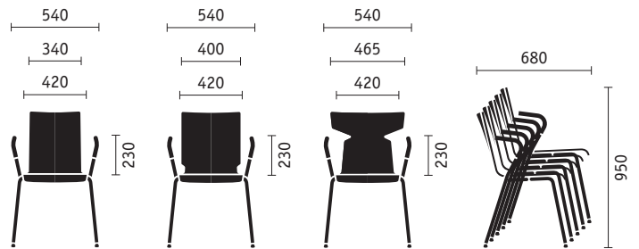
4-leg model with armrests integrated in the steel frame, straight-sided-, tailored- or T-shape one-piece shell, with seat and backrest cushion on request
